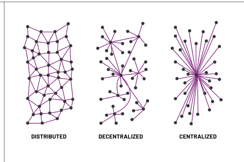
Figure 3 — Network architecture (adapted from Baran, 1962)
